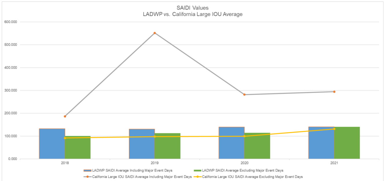
Figure 22: LADWP’s System Average Interruption Duration Index (2018-2021)
