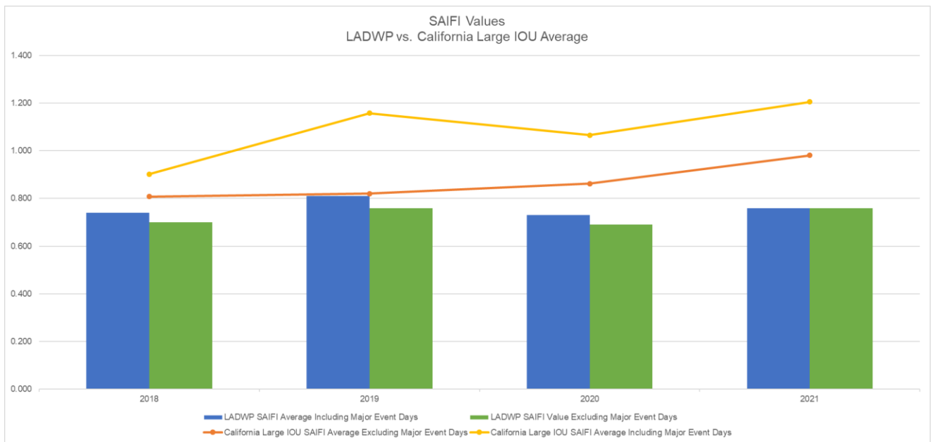
Figure 23: LADWP’s System Average Interruption Frequency Index (2018-2021)
