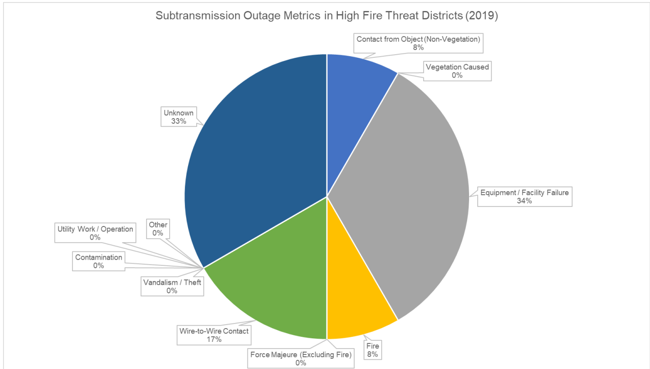
Figure 14: Subtransmission Outage Breakdown in HFTDs (2019)
