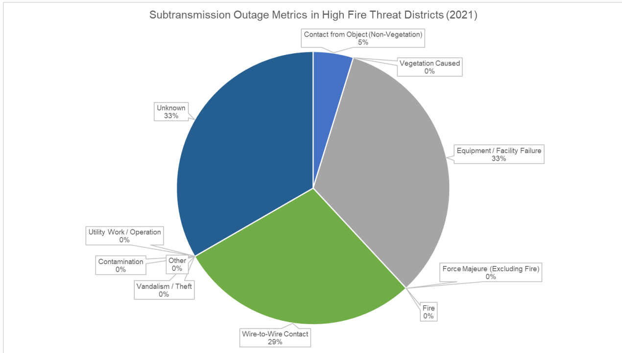
Figure 16: Subtransmission Outage Breakdown in HFTDs (2021)
