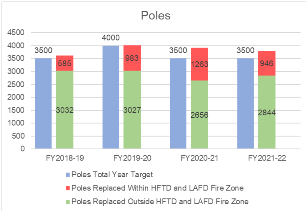
Figure 24: PSRP Pole Replacement
