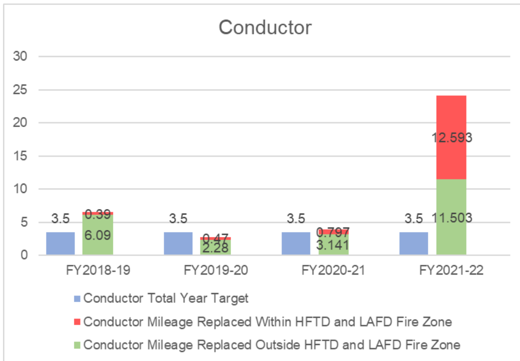
Figure 27: PSRP Conductor Mileage Replacement
